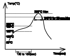
SMT temperature profile
