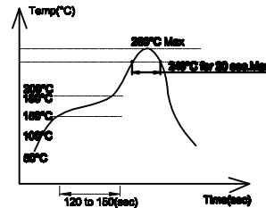
SMT temperature profile
